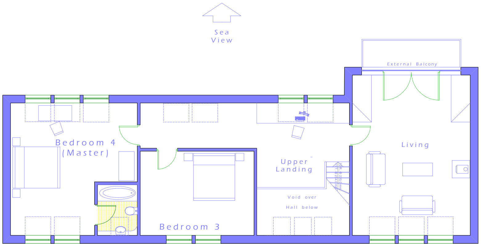
4-Bed Upper Floor Plan
